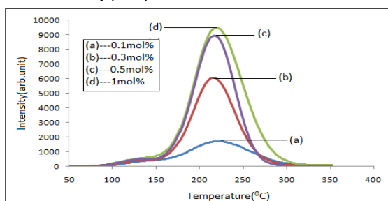
Fig. 7- TL glow curves of Na_2Sr_2Mg(BO_3)_2F_2:Eu^{3+} phosphor with different concentration of Eu^{3+} ions
