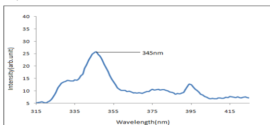
Fig. 5- Excitation spectrum of Na 2 Sr 2 Mg(BO 3 ) 2 F 2 :Eu 3+ phosphor
