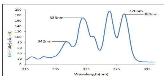
Fig. 2- Excitation spectrum of Na 2 Sr 2 Mg(BO 3 ) 2 F 2 :Tb 3+
