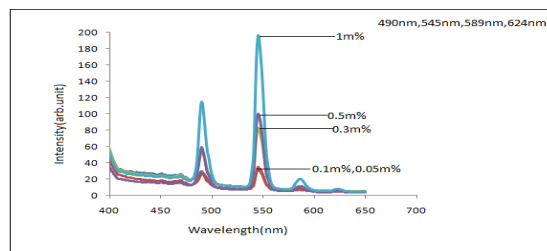
Fig. 3- Emission spectra of Na 2 Sr 2 Mg(BO 3 ) 2 F 2 :Tb 3+
