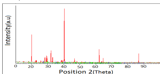
Fig. 1- X-ray powder diffraction pattern of Na 2 Sr 2 Mg(BO 3 ) 2 F 2 host
