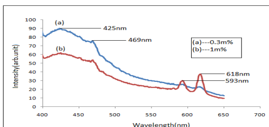
Fig. 6- Emission spectra of Na 2 Sr 2 Mg(BO 3 ) 2 F 2 :Eu 3+
