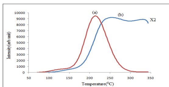
Fig. 8- Comparative glow curves of (a) Na_2Sr_2Mg(BO_3)_2F_2:Eu^{3+} and (b) CaSO_4:Dy
