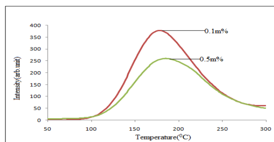
Fig. 10- TL glow curve of Na_2Sr_2Mg(BO_3)_2F_2:Tb^{3+}
