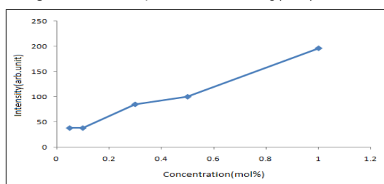
Fig. 4- Concentration of Tb 3+ ions vs PL peak intensity graph of Na 2 Sr 2 Mg(BO 3 ) 2 F 2 :Tb 3+ phosphor
