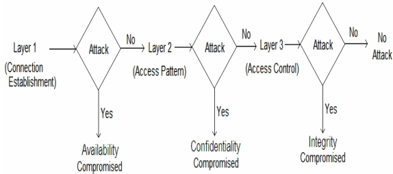
Fig. 1- Layered Approach
